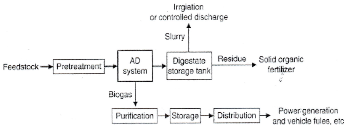
Figure : Layout of Biogas Plant
